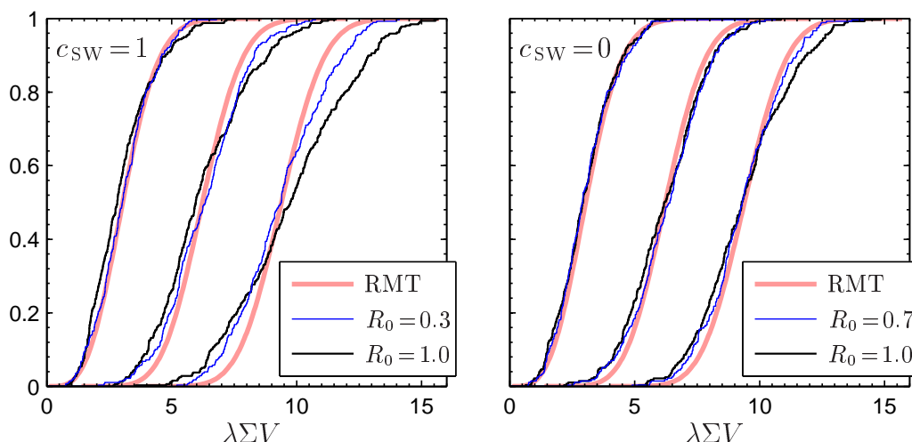
Figure 5: The cumulative distribution of the first three eigenmodes in the \nu = 1 topological sectors. Left panel: c_{\text{SW}} = 1 ; right panel: c_{\text{SW}} = 0 . The smooth thick lines are the RMT predictions.
